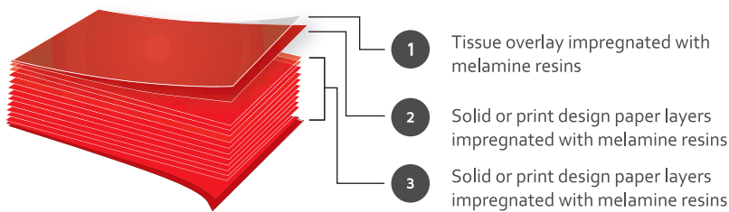
Unicore Compact Laminate Construction
